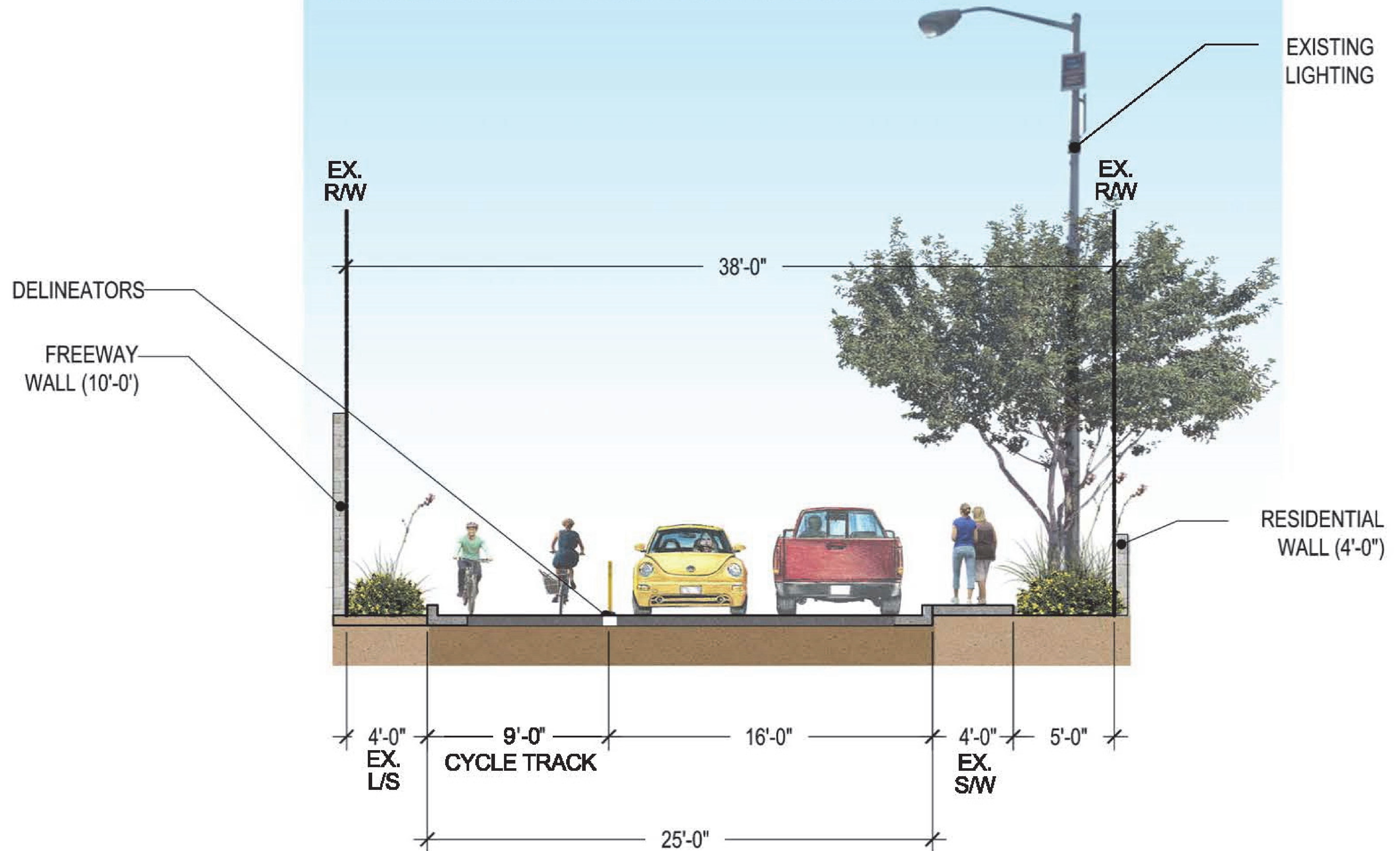
PROPOSED 38' ROW - 20TH PLACE W/ CYCLE TRACK
