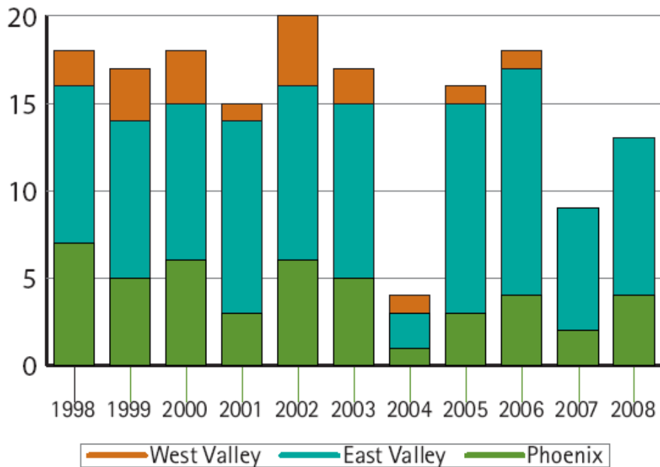
Total Ozone Exceedances in Maricopa County
