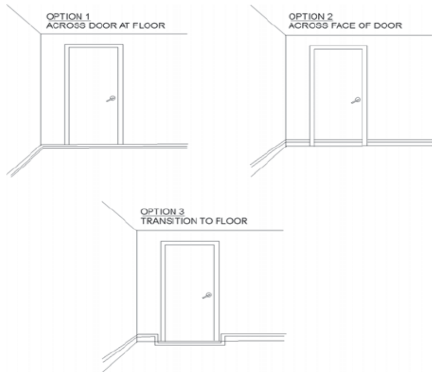
Figure 1024.2.4.3 PERIMETER DEMARCATION LINES— OPTIONS AT DOORS INTO EXIT ENCLOSURES
