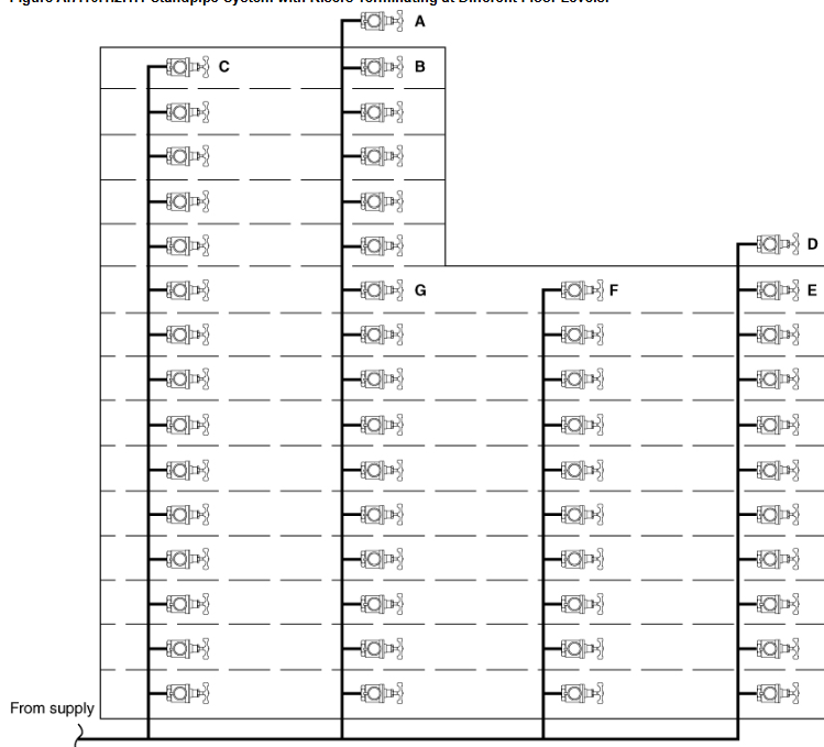
Figure A.7.10.1.2.1.1 Standpipe System with Risers Terminating at Different Floor Levels.
