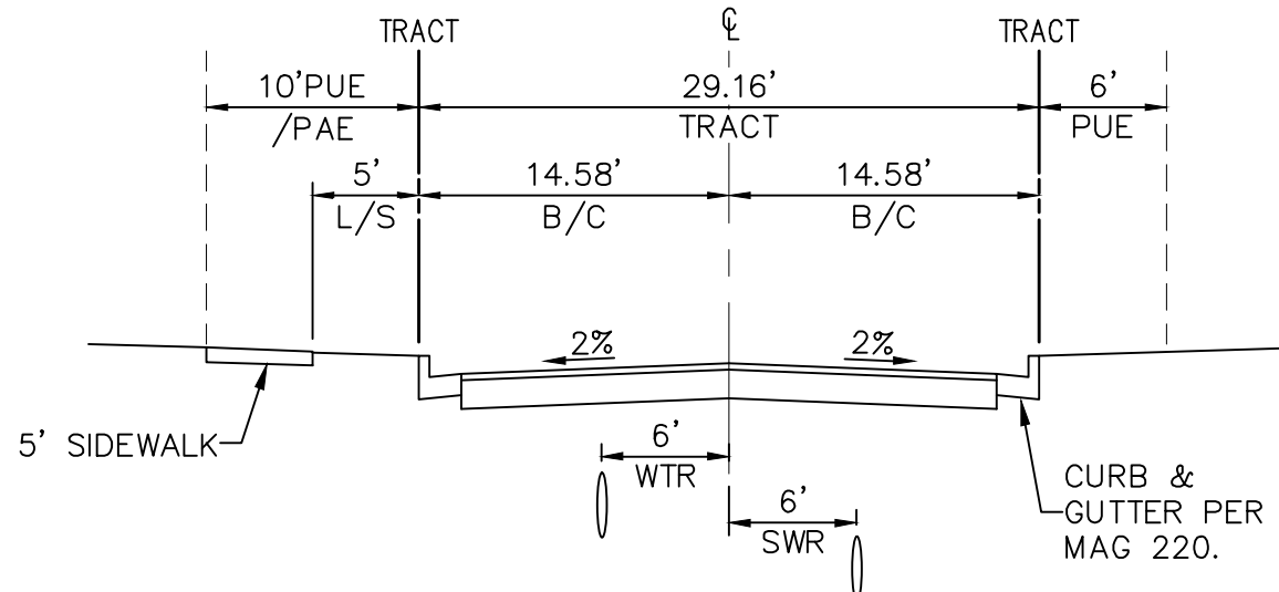
PRIVATE ACCESSWAY N.T.S.
