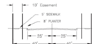
CROSS SECTION E 50/80
