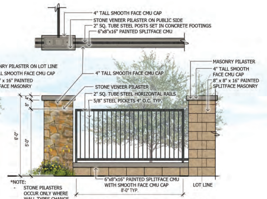
4 Full View Fence with Stone & Masonry Pilaster SCALE: 1/2"=1'-0"
