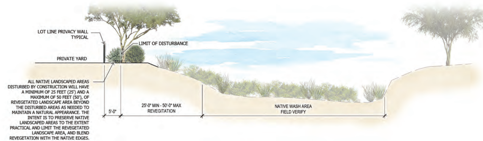
C Wash Edge Condition Cross Section SCALE: 1-1/2"=1'-0"
