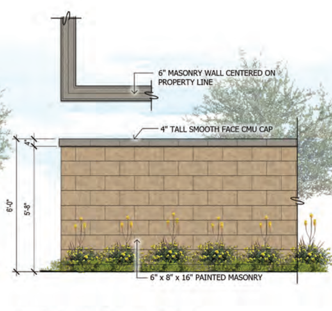
2 Secondary Theme Wall SCALE: 1/2"=1'-0"
