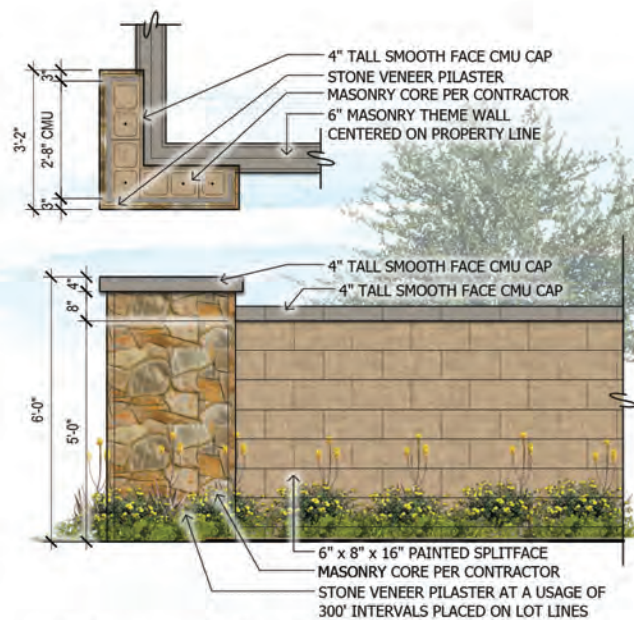
1 Perimeter Wall & Stone Pilaster SCALE: 1/2"=1'-0"
