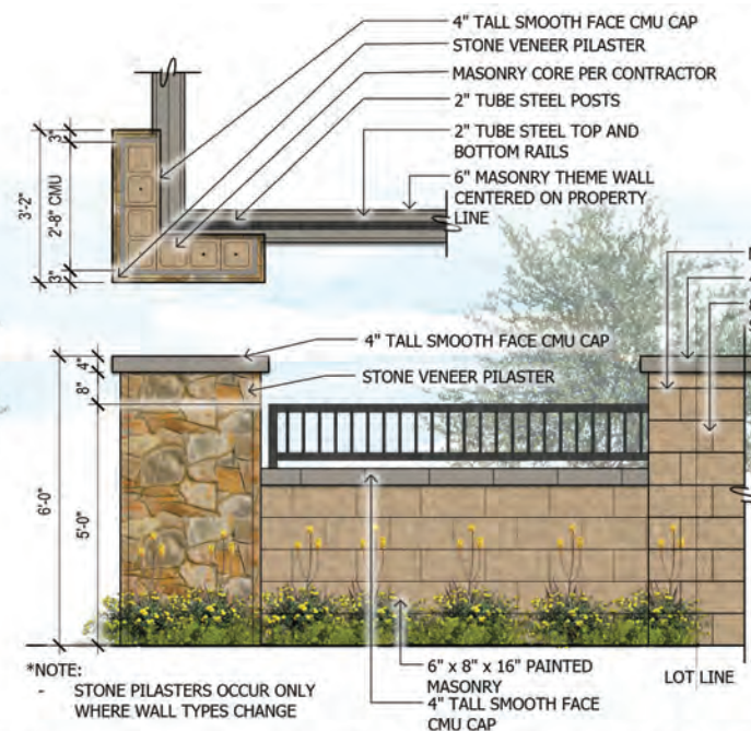
3 Partial View Fence with Stone & Masonry Pilaster SCALE: 1/2"=1'-0"
