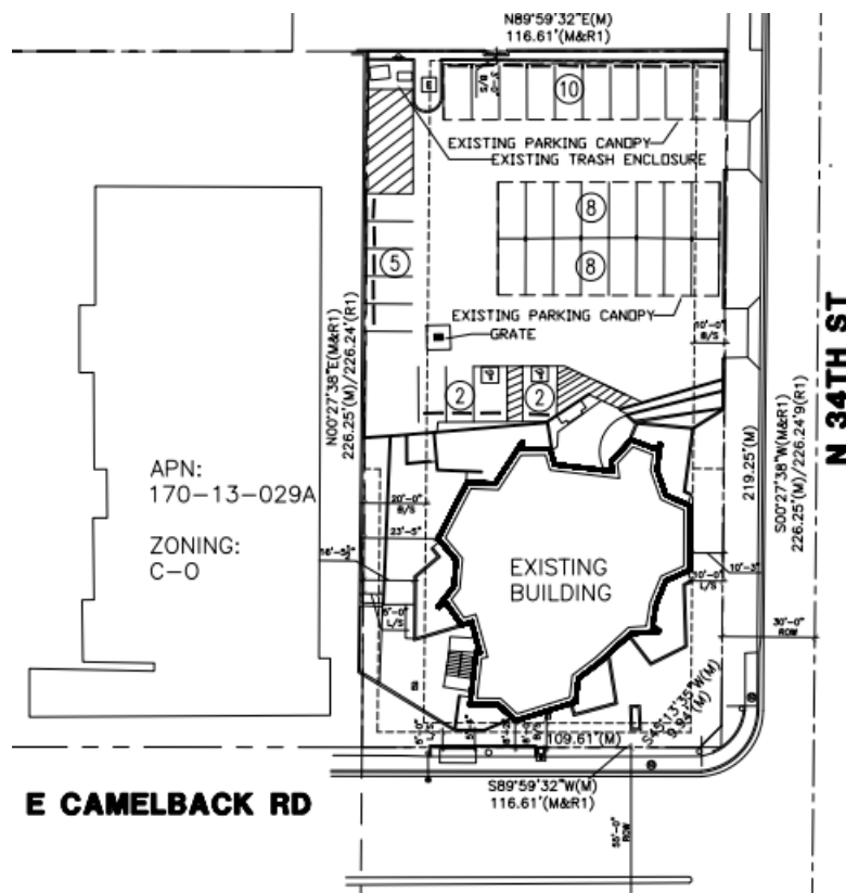
Figure 2 Site Plan
