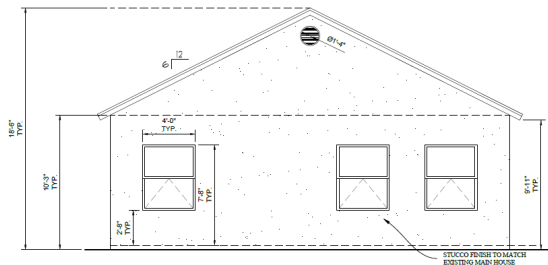
SIDE ELEVATION "D"
