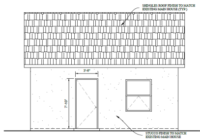
FRONT ELEVATION "A"
