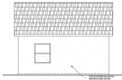
REAR ELEVATION "C"
