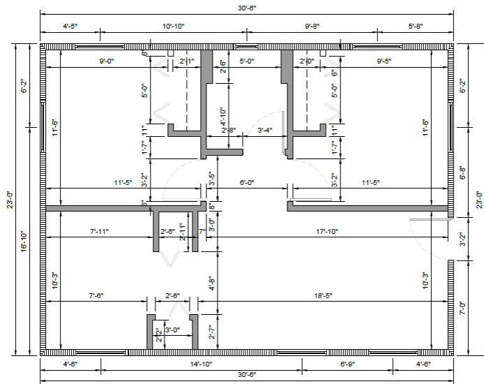
DIMENSION FLOOR PLAN
