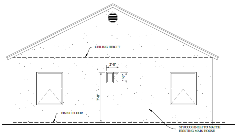
SIDE ELEVATION "B"
