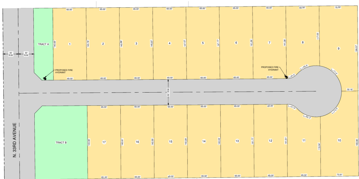
Conceptual Site Plan, Source: Diversified Future
