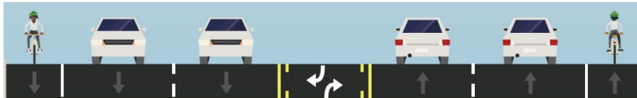
(Typical Cross Section)
