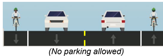
PROPOSED Travel Lanes on 65th PI / Montreal PI Greenway Pkwy to 66th St
