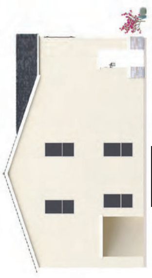
Left Elevation
