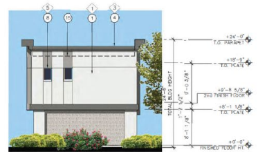
BUILDING TYPE 3 - RIGHT ELEVATION
