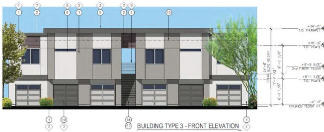
BUILDING TYPE 3 - FRONT ELEVATION
