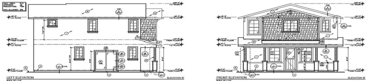
Conceptual Building Elevations, Source: 3 Engineering, LLC
