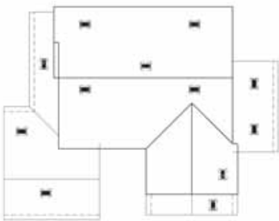
Roof Plan
